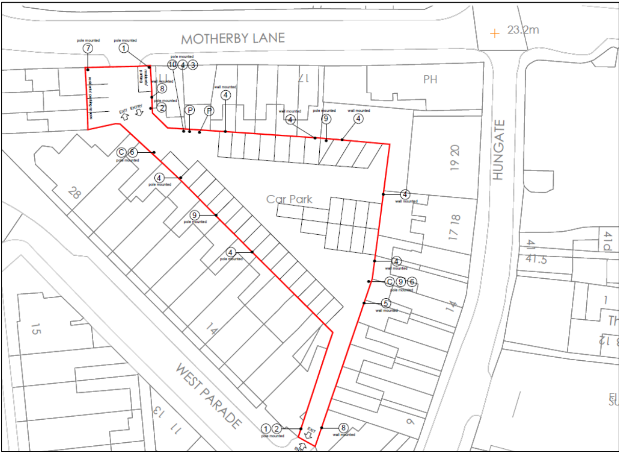
Site Plan
